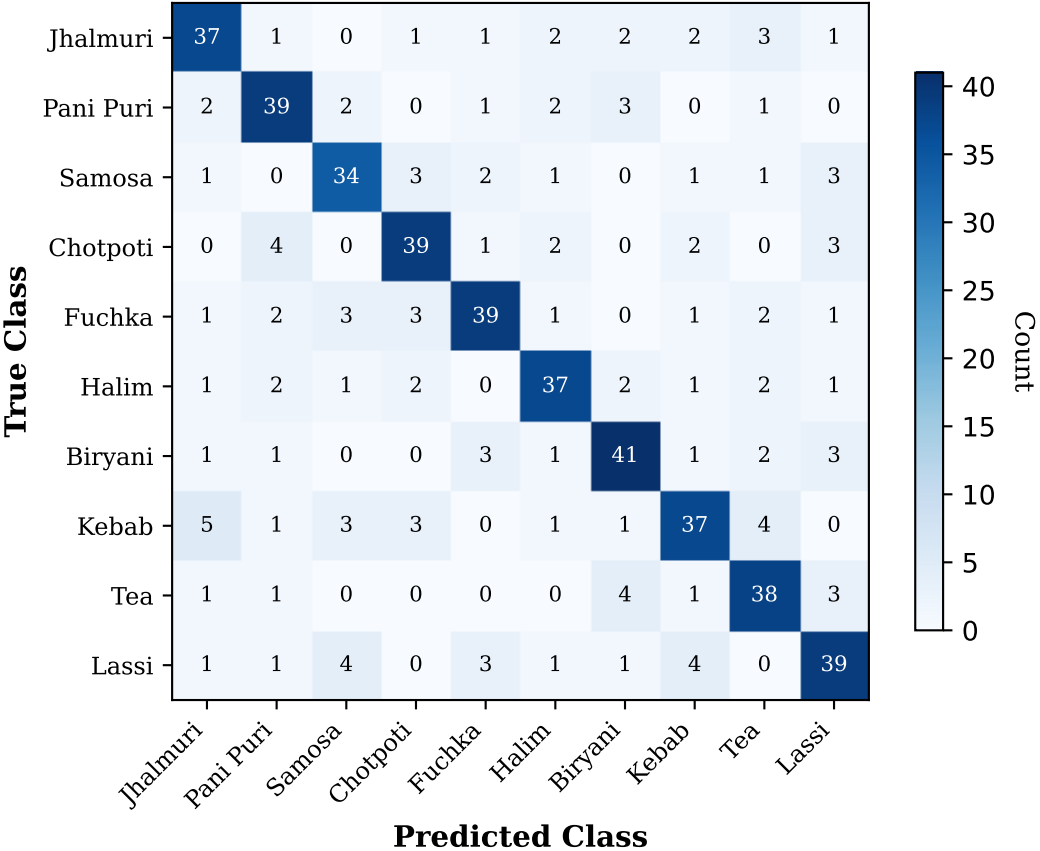
Confusion Matrix: YOLO11 Bangladesh Street Food Detection
